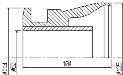
S4/001 campana / sleeve SD32 376+329
