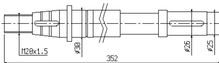
S4/058 albero / shaft SD63d121a
