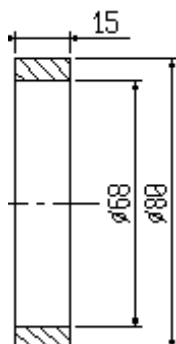
S4/008B anello / ring 383
