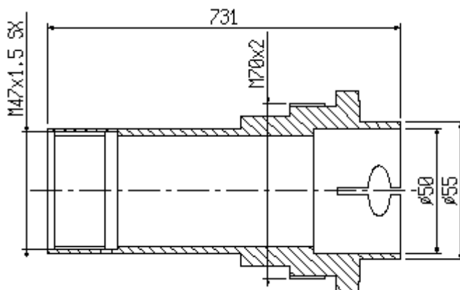
S4/010 tubo portapinza / collet tube 341
