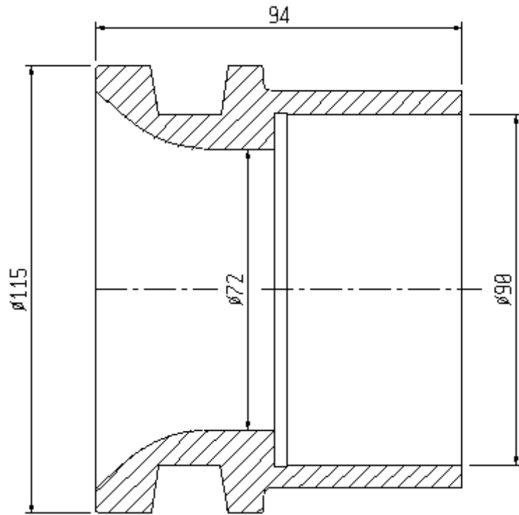
G12/001 Campana / sleeve 705-10-0016/001
