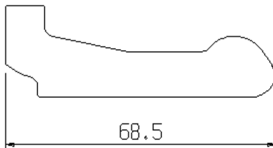
G12/003 martelletto / toggle 705-10-0017/001
