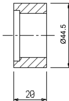
G9/030R rullo / roller 305-08-1420
