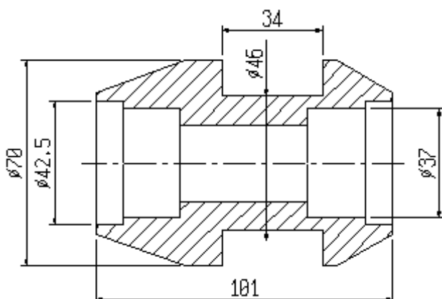
G9/050A rullo / roller
