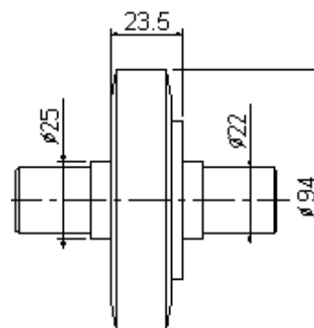
G2/040 rullo / roller
