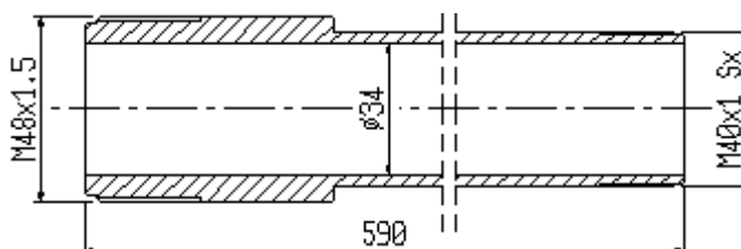
G2/010 tubo stringibarra / collet tube 351-10-217
