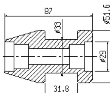
G3/050 rullo/roller 343-09-1370
