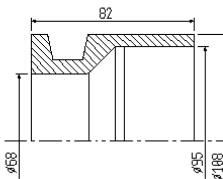
G2/002 campana/sleeve
