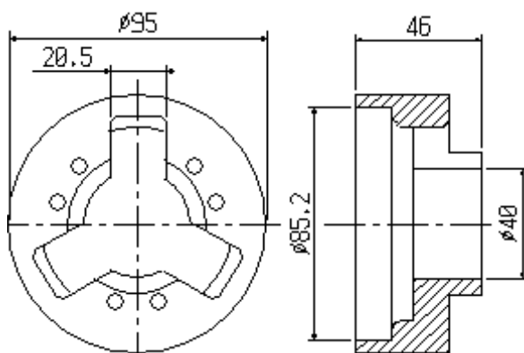
G2/011 mozzo/ring 341-10-214
