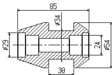
G4/050 rullo/roller
