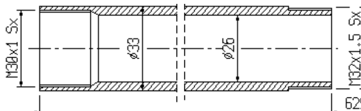
G2/012 tubo spingibarra / feed tube
